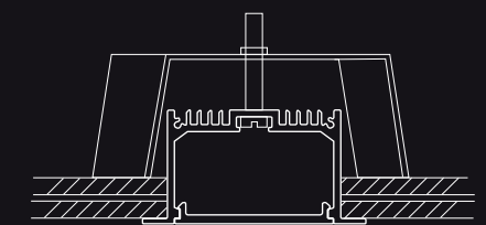
RECESSED 嵌入式
