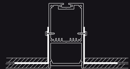
RECESSED 嵌入式
